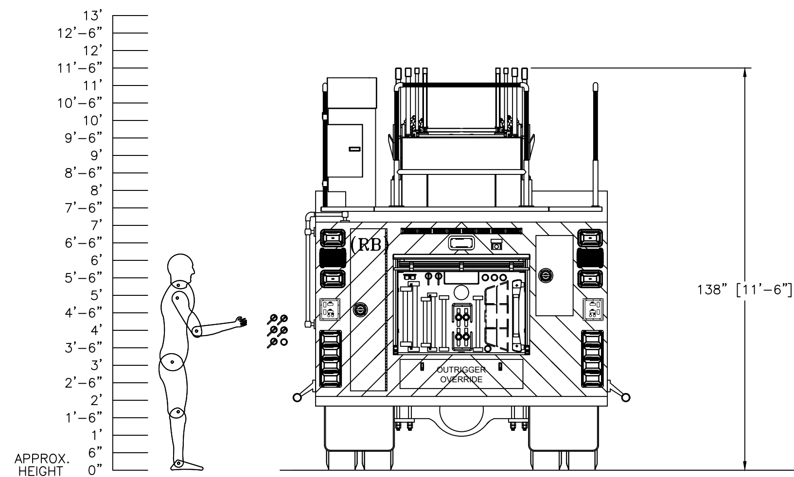
REAR VIEW
