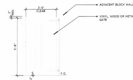
SIDE YARD GATE
