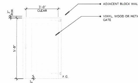
SIDE YARD GATE SCALE: 1/2"=1'-0" 24
