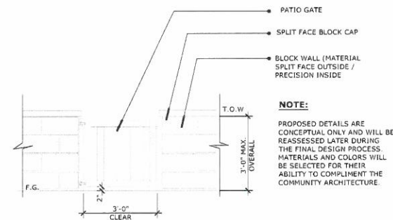
PATIO ENCLOSURE OPT. 3 - MASONRY
