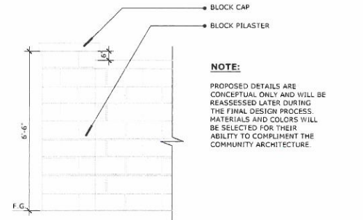
HIGH MASONRY PILASTER SCALE: 1/2"=1'-0" 24
