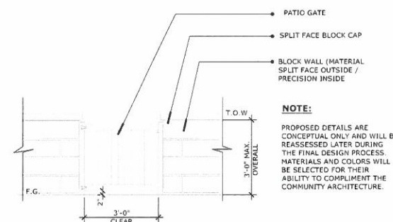
PATIO ENCLOSURE OPT. 3 - MASONRY
