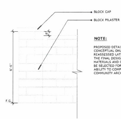
HIGH MASONRY PILASTER
