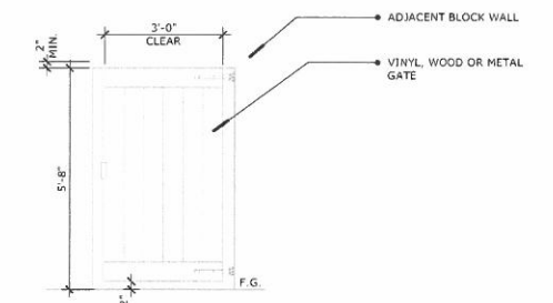
SIDE YARD GATE
