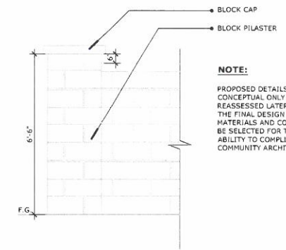
HIGH MASONRY PILASTER
