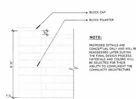
HIGH MASONRY PILASTER
