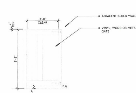
SIDE YARD GATE
