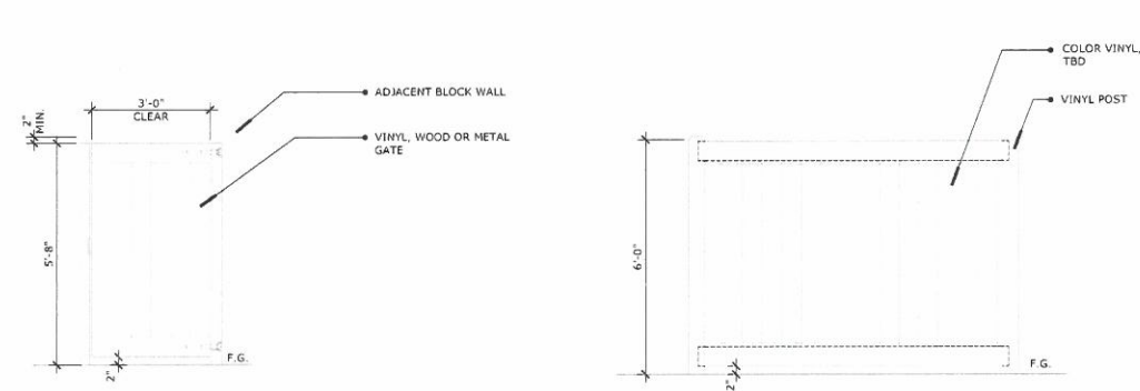
SIDE YARD GATE
