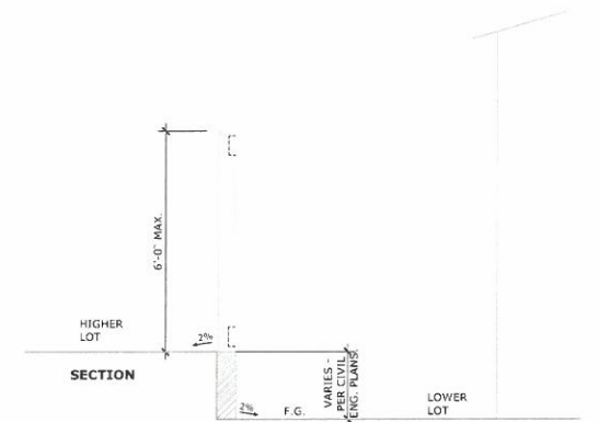
VINYL ON RETAINING WALL SECTION SCALE: 1/2"=1'-0"
