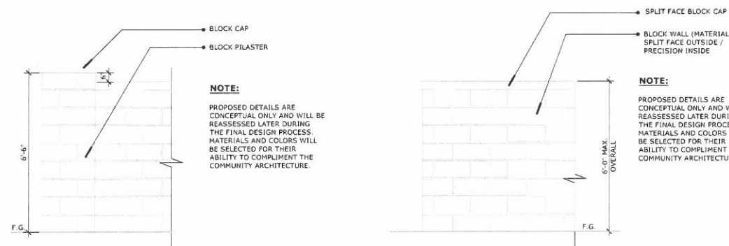
HIGH MASONRY PILASTER
