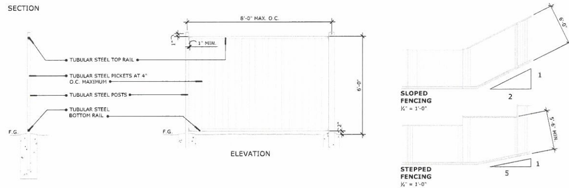
6'-0" HIGH T.S. FENCE
