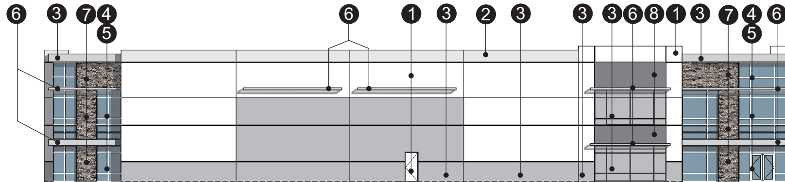
West Elevation
