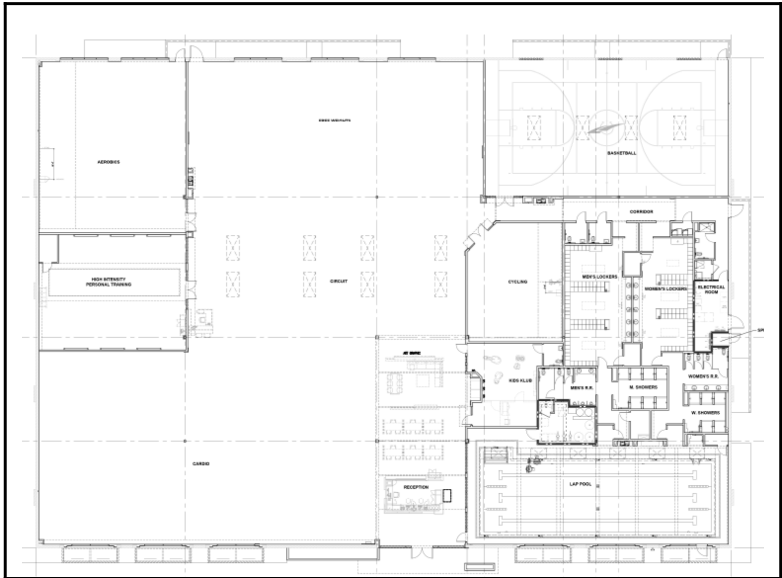
FLOOR PLAN
