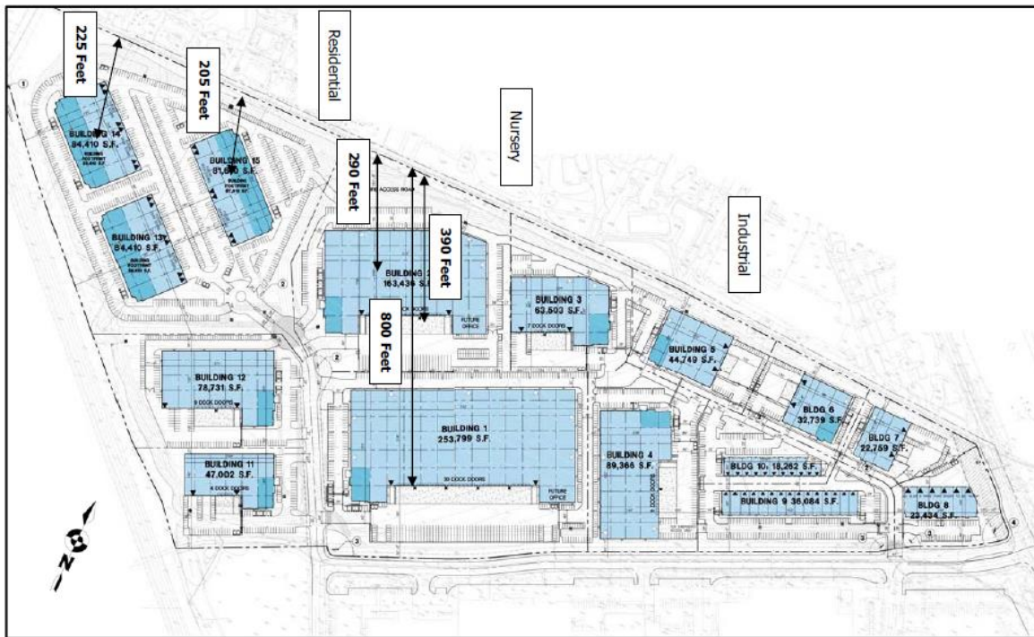
Figure 10-1 Stationary Sources
