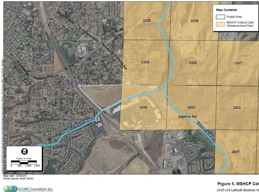
Figure 7-4 MSHCP Cells
